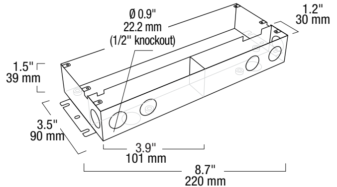
JUNCTION BOX
